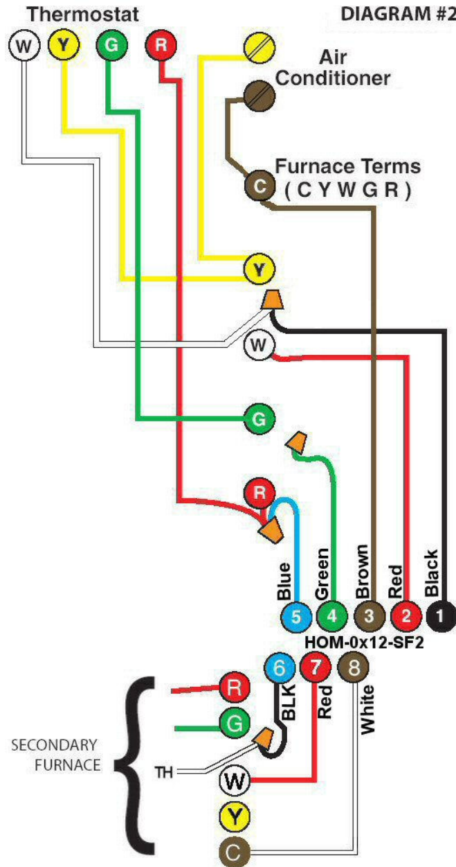
Diagram #2: Two Forced Air Furnaces having a common combustion air supply duct.
